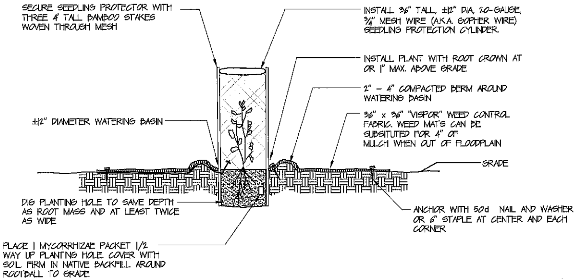
INSTALLATION ON FLAT GROUND
