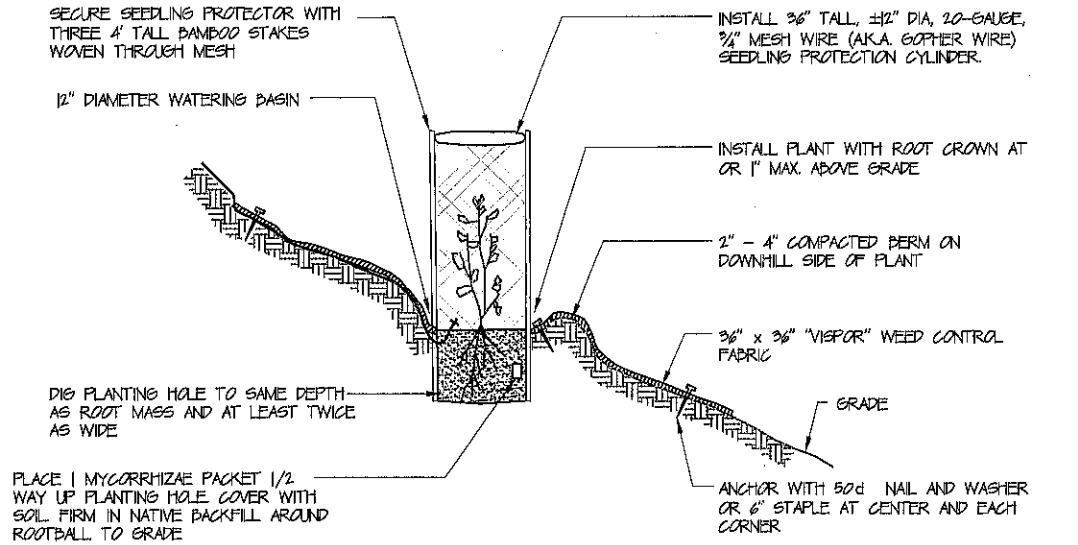
INSTALLATION ON HILL SLOPE
