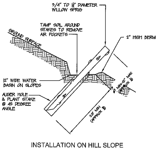
WILLOW & DOGWOOD STAKE PLANTING DETAIL
