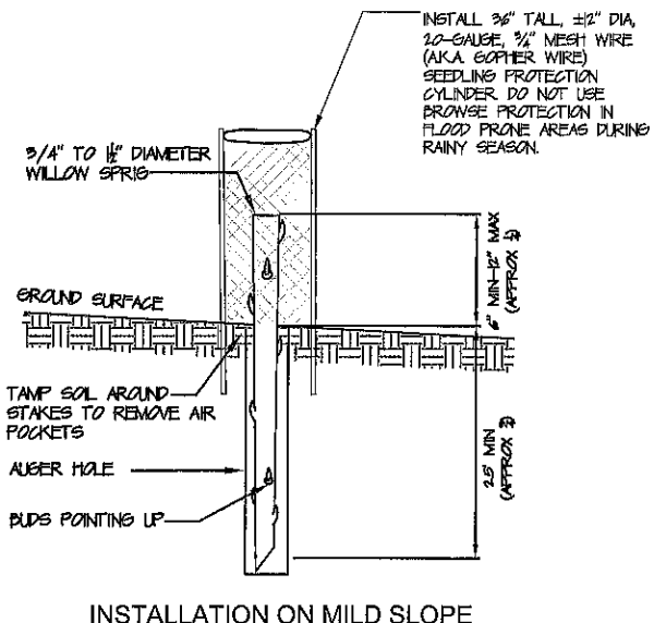
WILLOW & DOGWOOD STAKE PLANTING DETAIL
