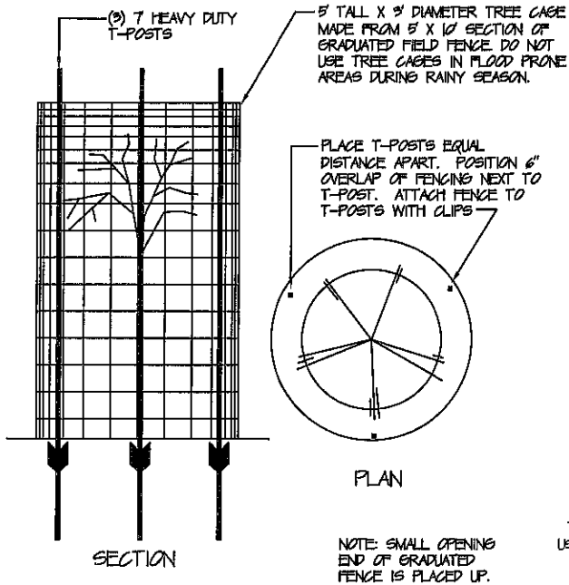
TREE CAGE DETAIL
