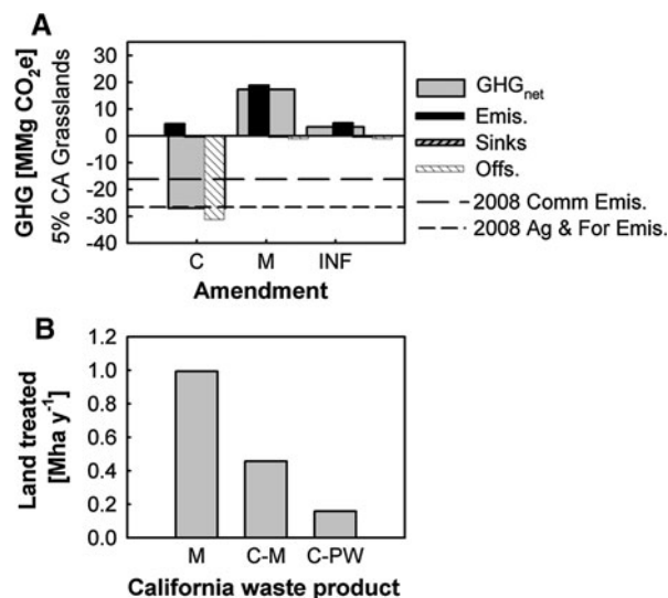
Figure 7. A Potential impacts of soil amendments on net greenhouse gas fluxes when applied over an area equal to 5% of California grasslands. Emissions from the California Agriculture and Forestry and Commercial Sectors (CARB 2011) are shown for comparison. B Area of land statewide that could potentially be treated annually using cattle manure (M), composted manure (C-M), or composted plant waste (C-PW) assuming application rates used in the initial case study (Table 3) and material availability (Table 4).
